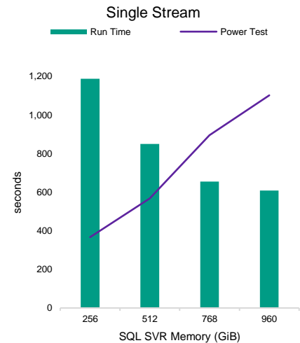
Figure 4: Single-stream performance
