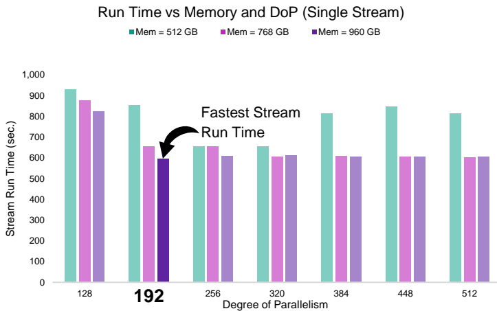
Figure 2: Single-stream DoP
