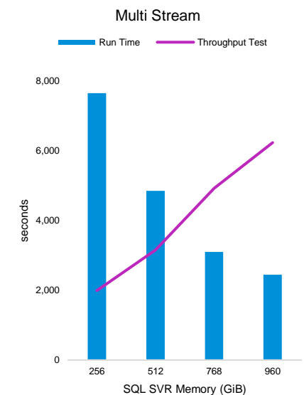
Figure 5: Multi-stream performance
